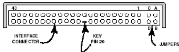
Figure 1.HDD Jumper Locations
